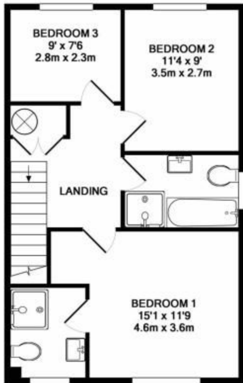
1ST FLOOR
